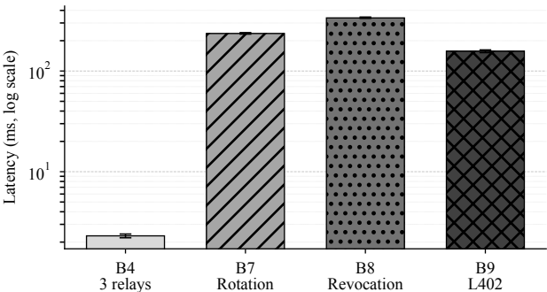
Docker Infrastructure Benchmarks
