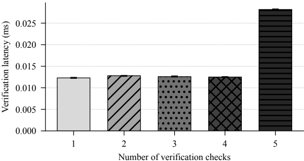
SP-5: L402 Check Ablation
