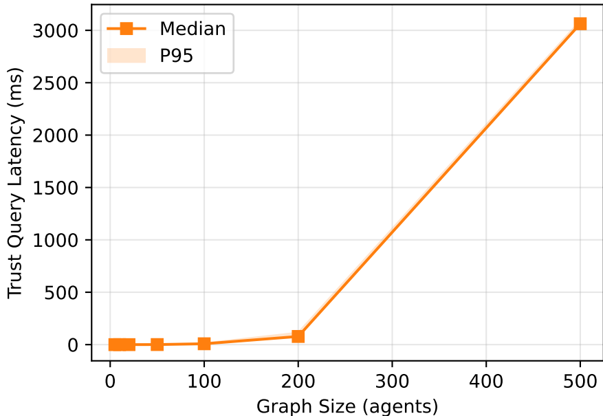
B6: Trust Graph Size vs. Query Latency
