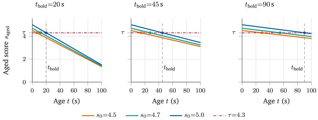
Figure 10: Linear aging of the FIM score at three hold-times. Each panel shows the same scores s_0 \in \{4.5, 4.7, 5.0\} ; the vertical line is t_{\text{hold}} , where a score-5 thought crosses \tau . Within a panel, weaker thoughts expire sooner. Left to right, a shorter t_{\text{hold}} steepens every line. Parameters: \tau = 4.3 , s_{\text{hold}} = 5 . – Source: Own illustration .
