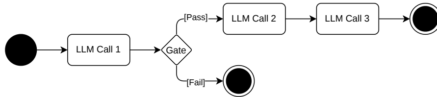
Figure 3: Prompt chaining: A complex task is decomposed into sequential LLM calls – Source: Own illustration based on "Building Effective AI Agents by Anthropic"[34], created with draw.io.
