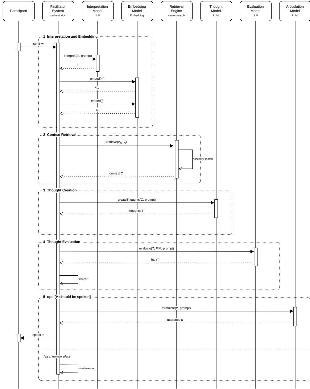
Figure 11: Thought Pipeline Sequence: Sequence of the thought pipeline – Source: Own illustration based on “Inner Thoughts” by Liu et al.[36], created with draw.io.
