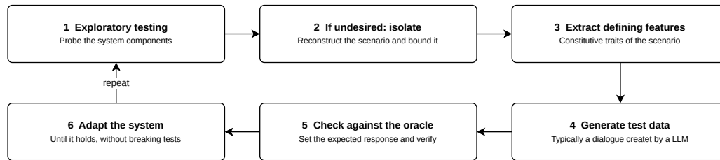
Figure 8: Evaluation-driven development loop: From exploratory testing to system adaptation – Source: Own illustration, created with draw.io.
