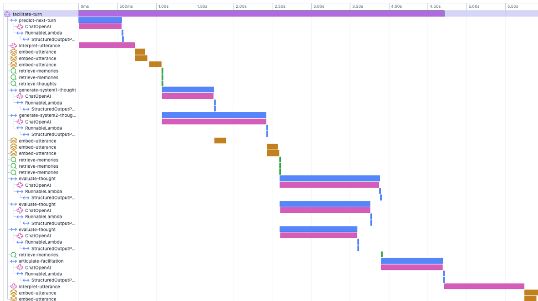
Figure 9: Langfuse: Screenshot of the Traceviewer in Langfuse that shows the trace of the AI-Facilitator processing a new conversation event. – Source: Own screenshot, created with Langfuse.
