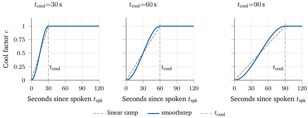
Figure 11: Cooldown factor after a thought is spoken, for t_{\text{cool}} \in \{30, 60, 90\} s. Each panel compares the Hermite smoothstep with a linear ramp; the vertical line is t_{\text{cool}} , where recovery completes. The smoothstep stays flat at both ends; the linear ramp starts immediately and kinks at t_{\text{cool}} . – Source: Own illustration, created with LaTeX and TikZ
