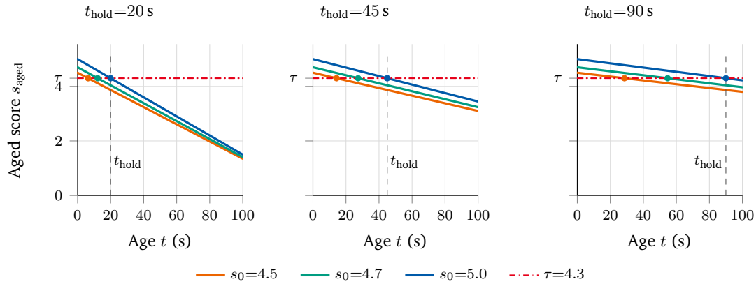
Figure 10: Linear aging of the FIM score at three hold-times. Each panel shows the same scores s_0 \in \{4.5, 4.7, 5.0\} ; the vertical line is t_{\text{hold}} , where a score-5 thought crosses \tau . Within a panel, weaker thoughts expire sooner. Left to right, a shorter t_{\text{hold}} steepens every line. Parameters: \tau = 4.3 , s_{\text{hold}} = 5 . – Source: Own illustration, created with LaTeX and TikZ
