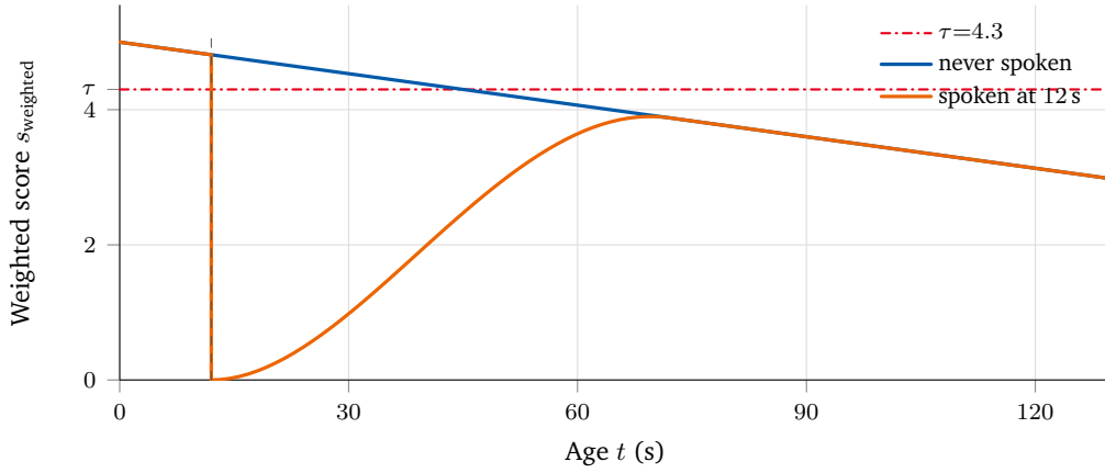
Figure 12: Weighted FIM score of a thought with s_0 = 5 , never spoken versus spoken at t = 12 s. Aging uses t_{\text{hold}} = 45 s; cooldown uses t_{\text{cool}} = 60 s. Recovery restores the aged remainder; whether that remainder still exceeds \tau depends on how long the thought has already lived. Parameters: \tau = 4.3 , s_{\text{hold}} = 5 . – Source: Own illustration, created with LaTeX and TikZ
