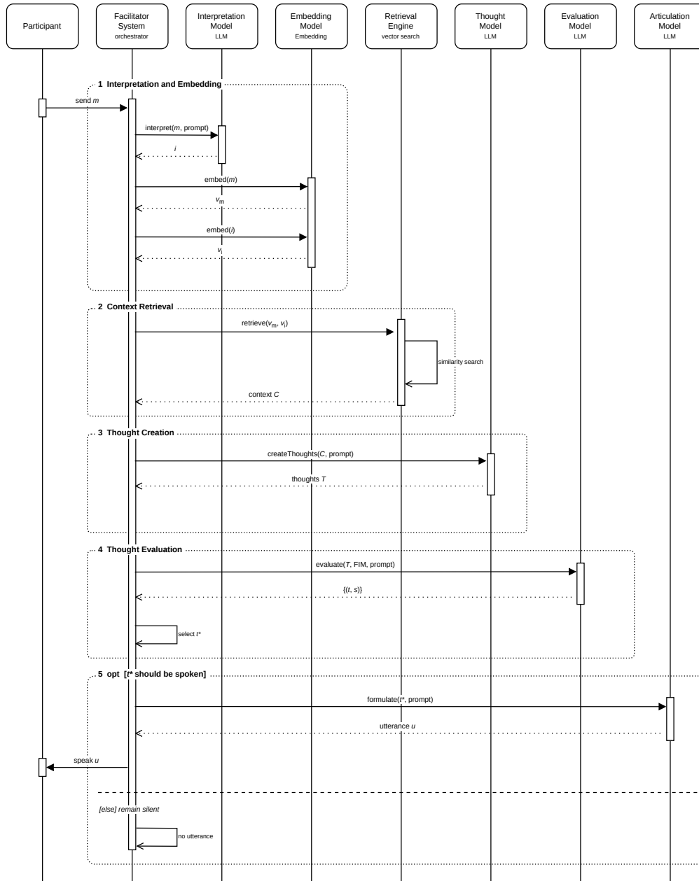
Figure 9: Thought Pipeline Sequence: Sequence of the thought pipeline – Source: Own illustration based on “Inner Thoughts” by Liu et al.[33], created with draw.io.
