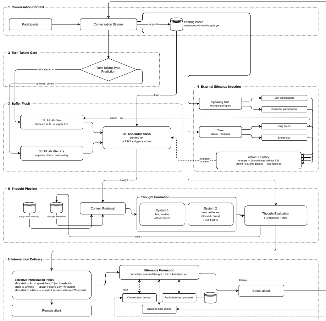
Figure 8: System Architecture: Adapted version of the “Inner Thoughts” framework – Source: Own illustration based on “Inner Thoughts” by Liu et al.[36], created with draw.io.
