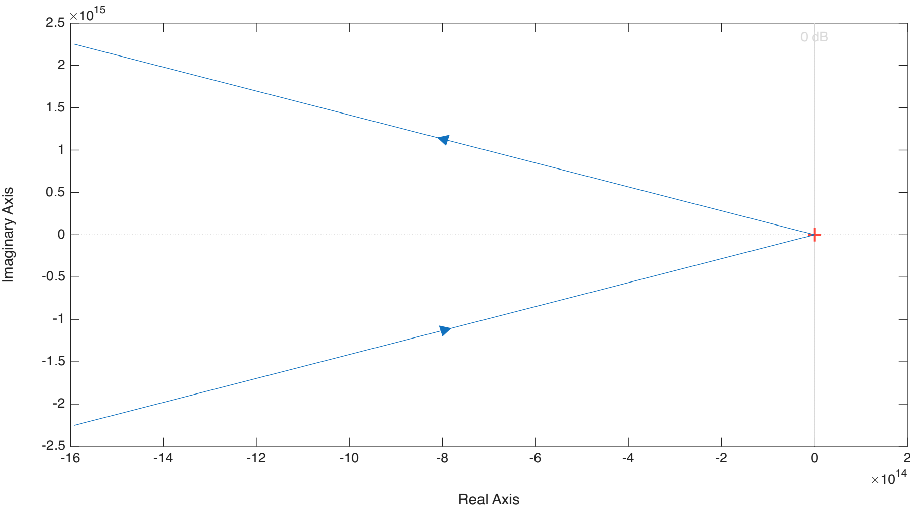
Nyquist Plot of PC(s) = (s+2)/(s(s^2+2))
