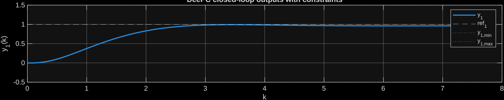
DeePC closed-loop outputs with constraints
