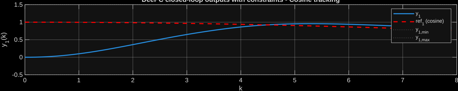
DeePC closed-loop outputs with constraints - Cosine tracking
