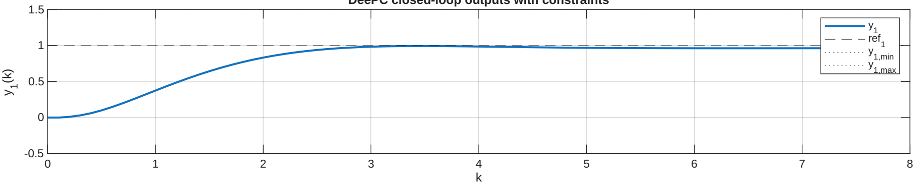
DeePC closed-loop outputs with constraints
