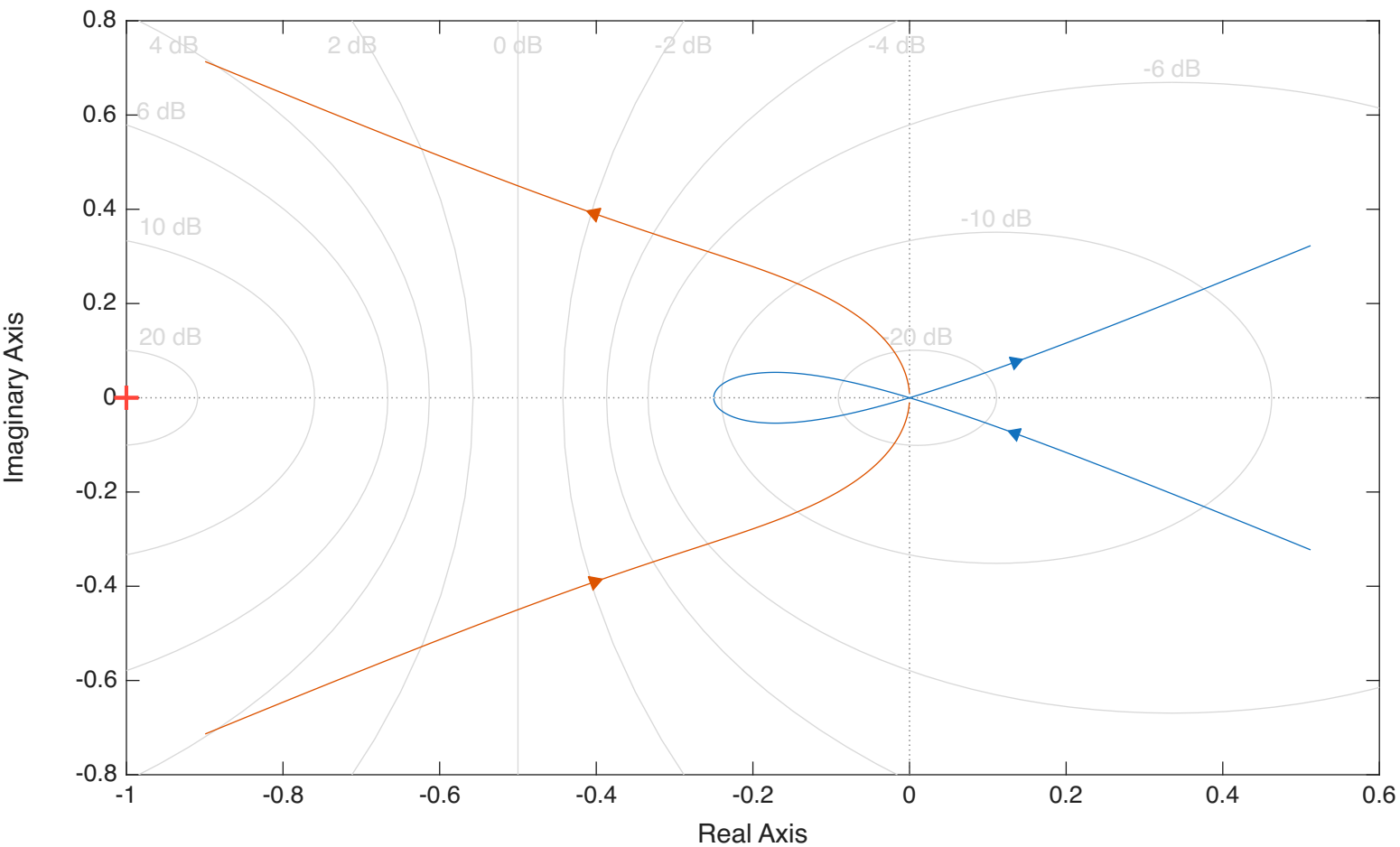
Nyquist plot of P(s) = (s^2+1)/((s^2+2)(s-2))
