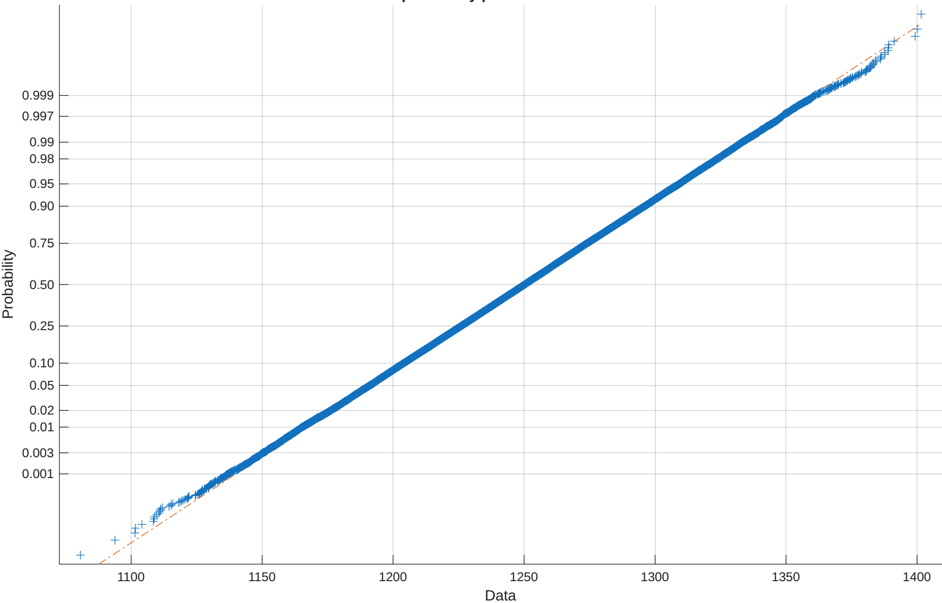
Normal probability plot for the LS estimates
