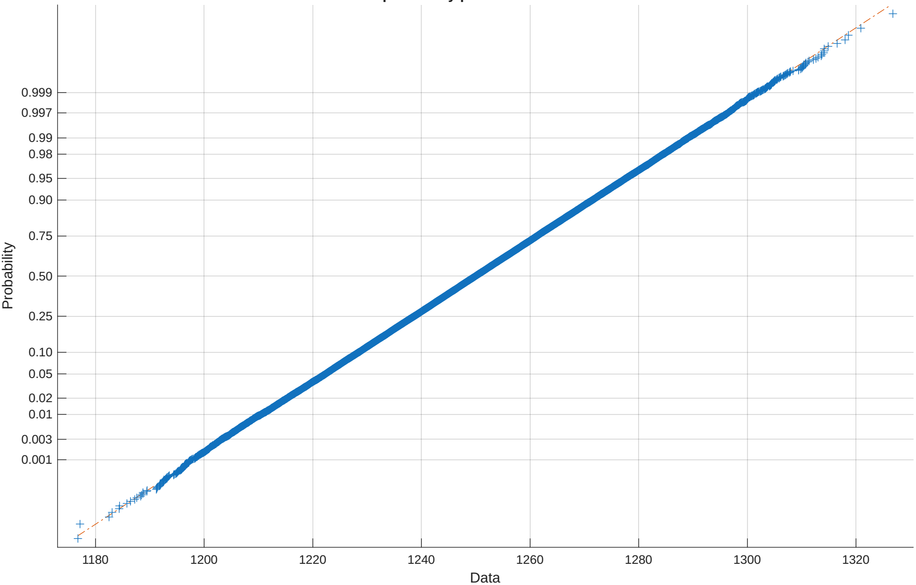
Normal probability plot for the WLS estimates
