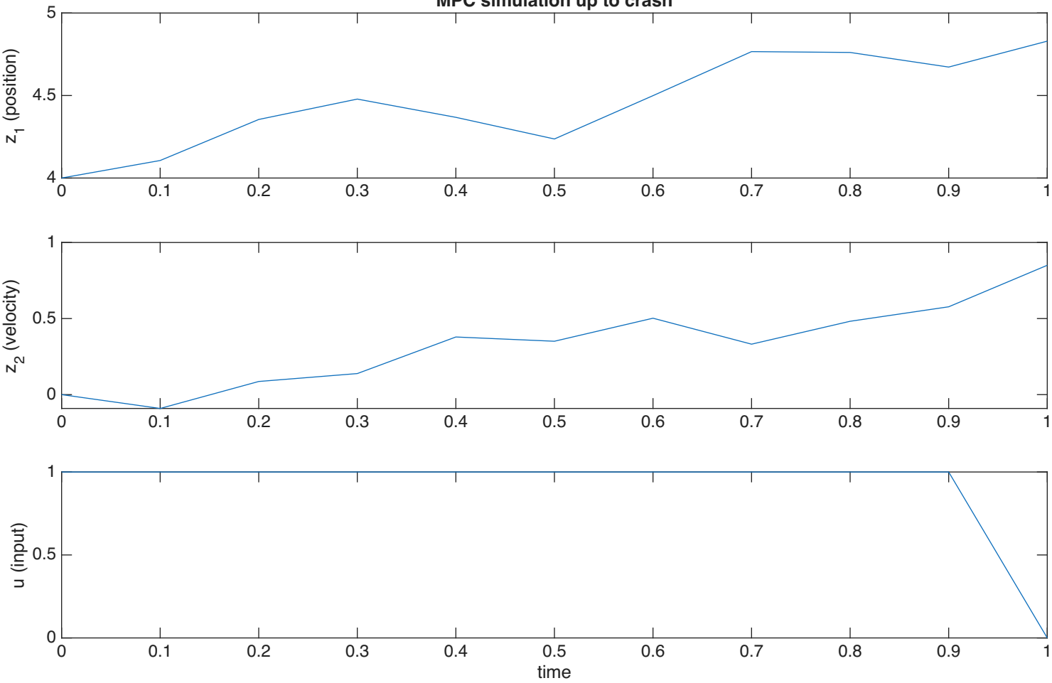
MPC simulation up to crash
