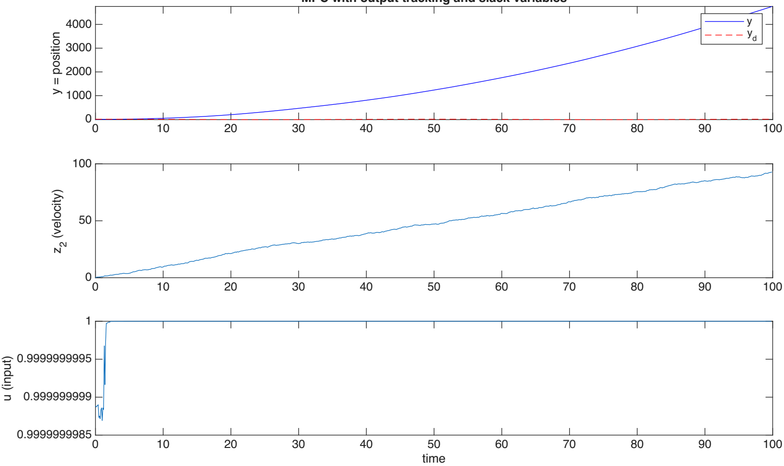
MPC with output tracking and slack variables
