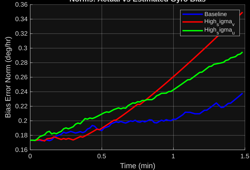
Norms: Actual vs Estimated Gyro Bias
