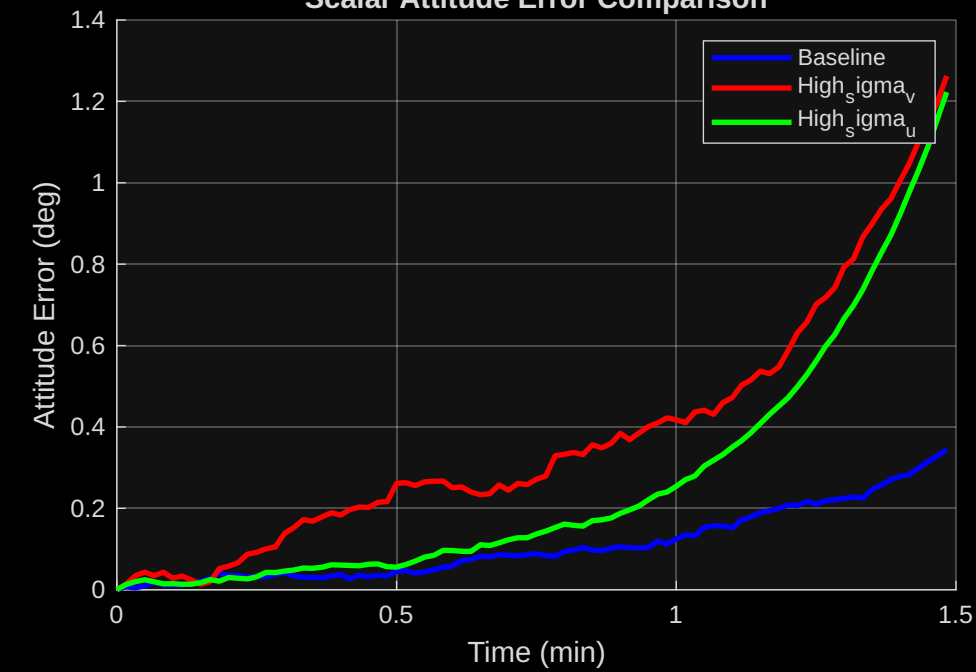
Scalar Attitude Error Comparison
