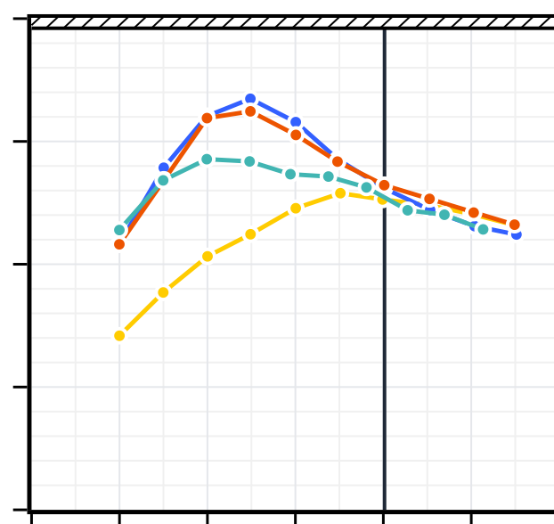
Simplicial Complex
