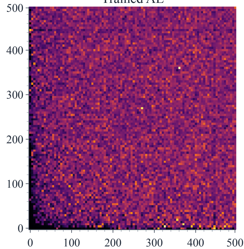
Trained AE
