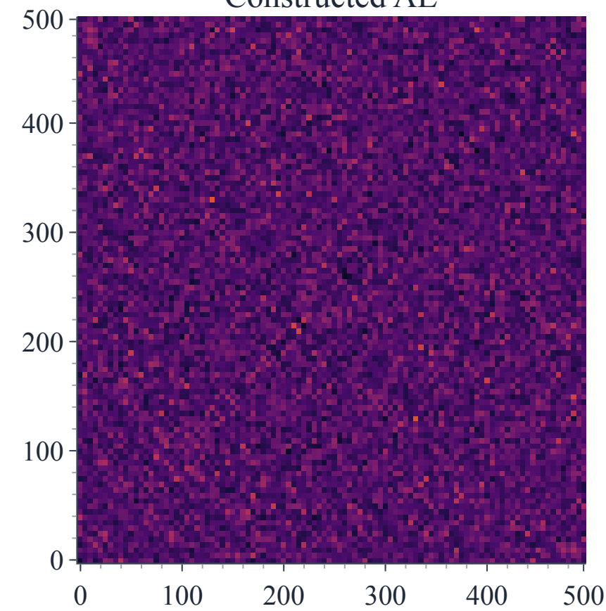
Constructed AE
