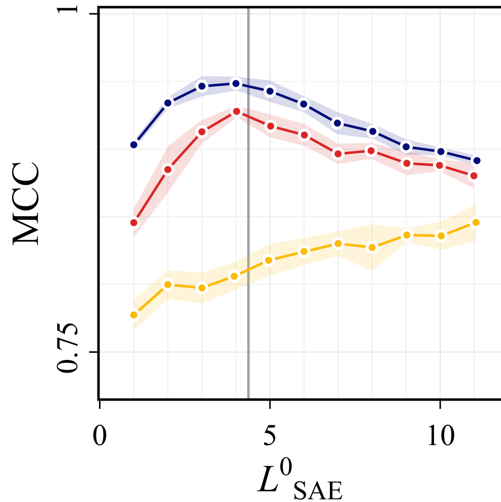
ReLU SAE(Trained AE w/ Unit Norms)
