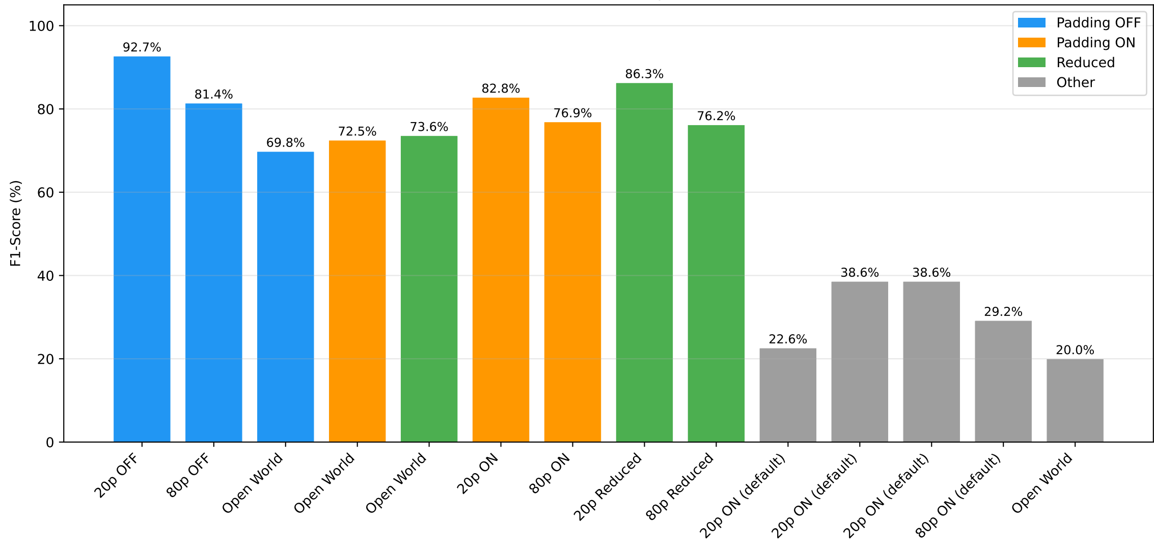
F1-Score Across All Experiments
