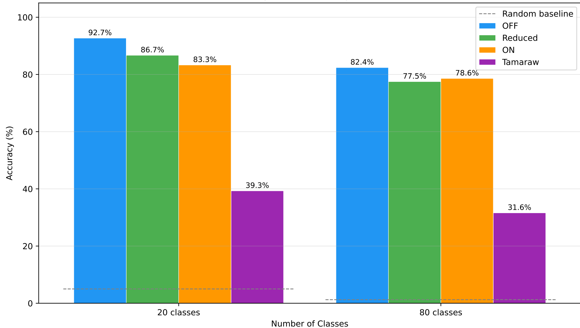
DF Accuracy: Circuit Padding vs Tamaraw
