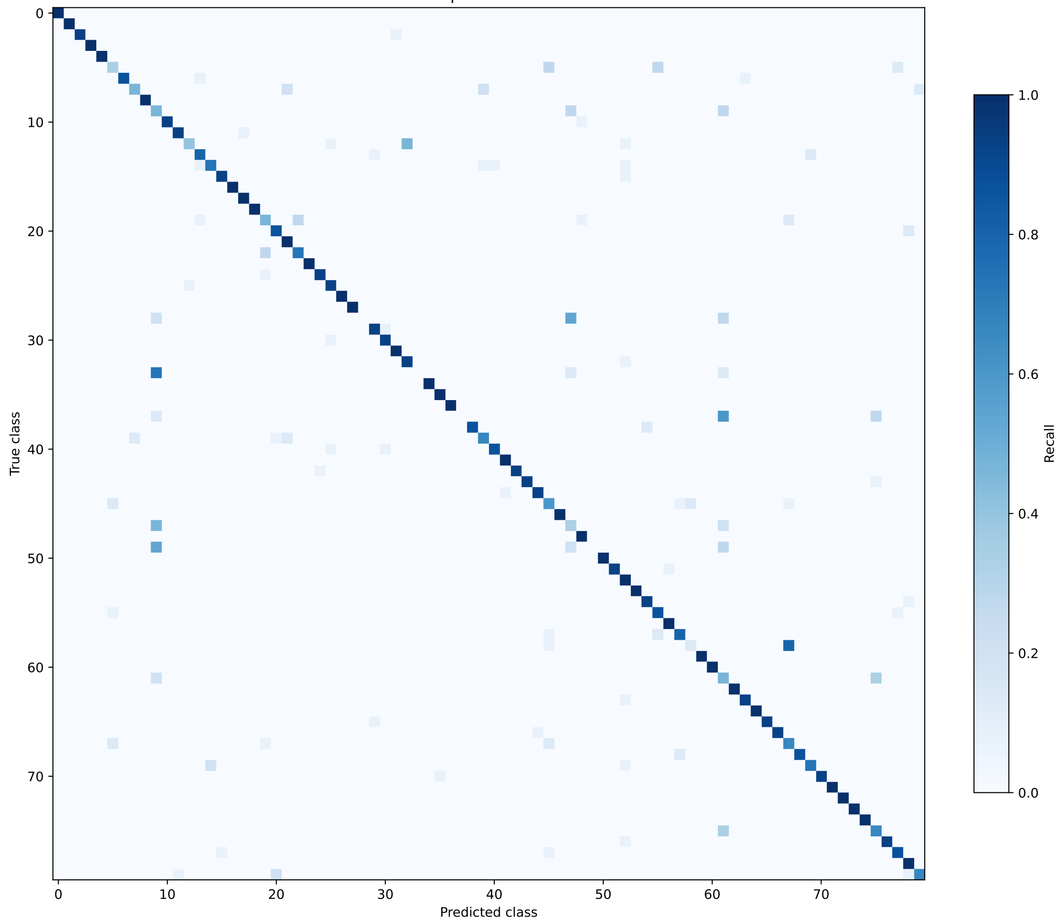
ExpBaseline80
