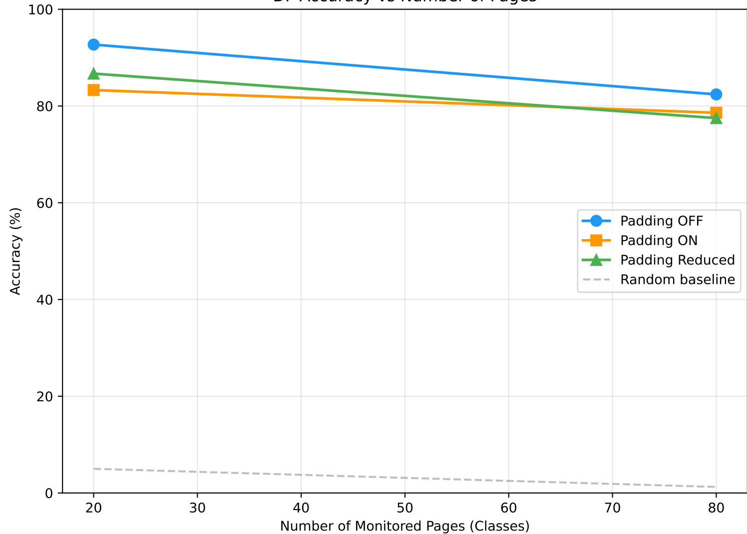
DF Accuracy vs Number of Pages
