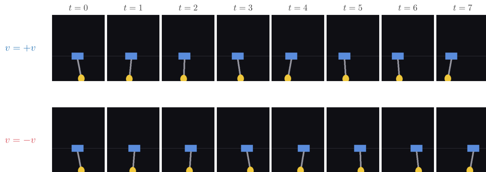
CartPole (wider/deeper CNN backbone ablation): same configuration, opposite velocity (Protocol B kill experiment)
