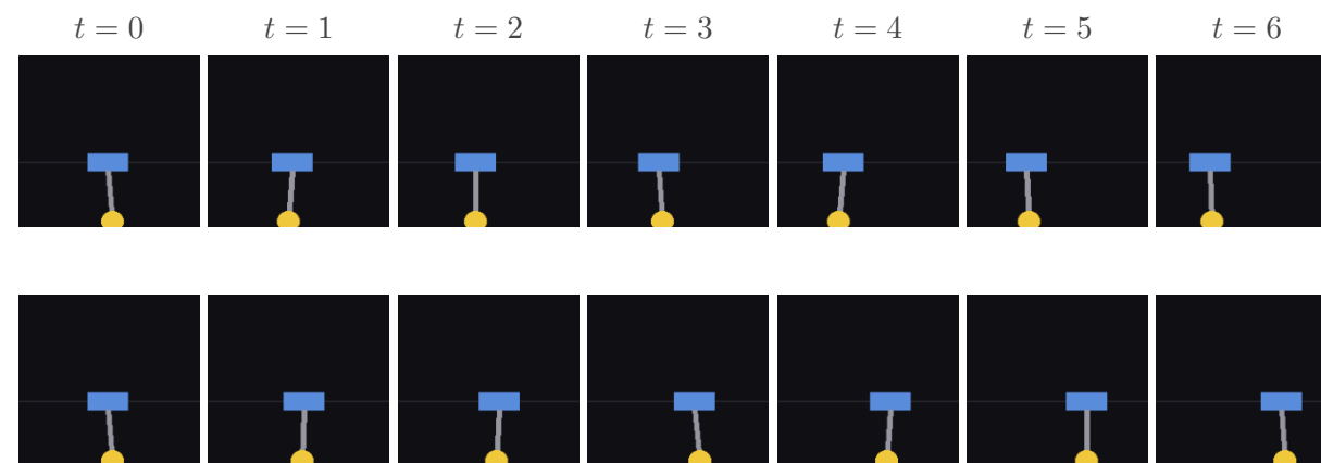
CartPole
