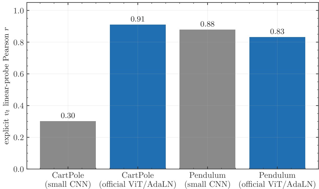
Switching encoder family closes CartPole's small-CNN gap
