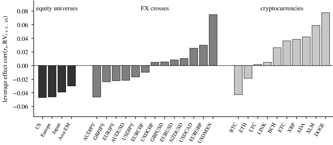
Figure 9. The leverage effect per instrument, grouped by venue class: the four equity-universe estimates, the 13 FX crosses, and the 10 registered cryptocurrencies, each sorted within its group. Every equity universe is negative; the FX crosses scatter symmetrically about zero along the flight-to-quality axis; the coins are predominantly positive, with BTC and ETH the exceptions.
