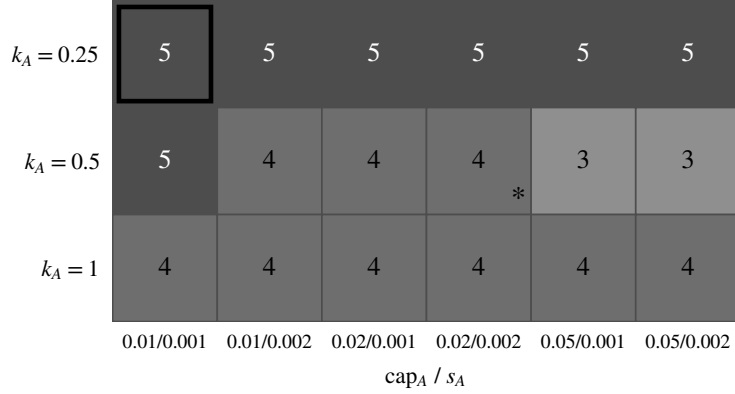
Figure 3. The Experiment I tuning grid (tuning seeds 900–903, disjoint from evaluation): battery score by anticipator response k_A , capital \text{cap}_A , and execution-noise scale s_A . Darker cells score higher. The score is non-increasing in every strengthening direction; the tied best settings are the weakest anticipators. The heavy box marks the tie-break selection (the frozen evaluation setting); the asterisk marks the pre-registered first-shot setting.
