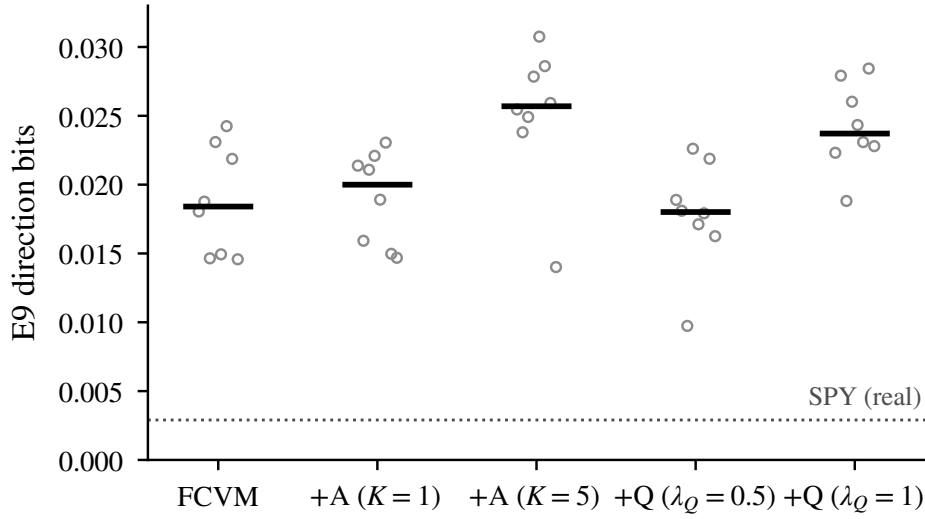
Figure 4. E9 direction bits across every rationality configuration (open circles: evaluation seeds; bars: medians). No configuration approaches the information-free regime; real SPY (dotted, 0.0029) sits far below all of them. Trading against the flow, iterating that trade to depth five, and absorbing the flow’s impact into the price level all leave the sign channel open or wider.
