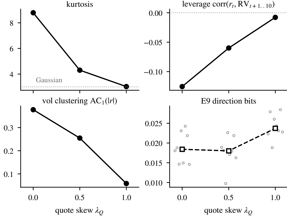
Figure 3. Wild-fact medians versus quote skew \lambda_Q (8 evaluation seeds). Full absorption of the forecastable flow’s price impact kills the fat tails (kurtosis 8.8 \rightarrow 3.0 ), the leverage effect ( -0.125 \rightarrow -0.008 ) and volatility clustering ( \text{AC}_1(|r|) 0.38 \rightarrow 0.06 ) — while the E9 direction bits (bottom right; open circles are seeds) do not close: flat at half skew, higher at full skew.
