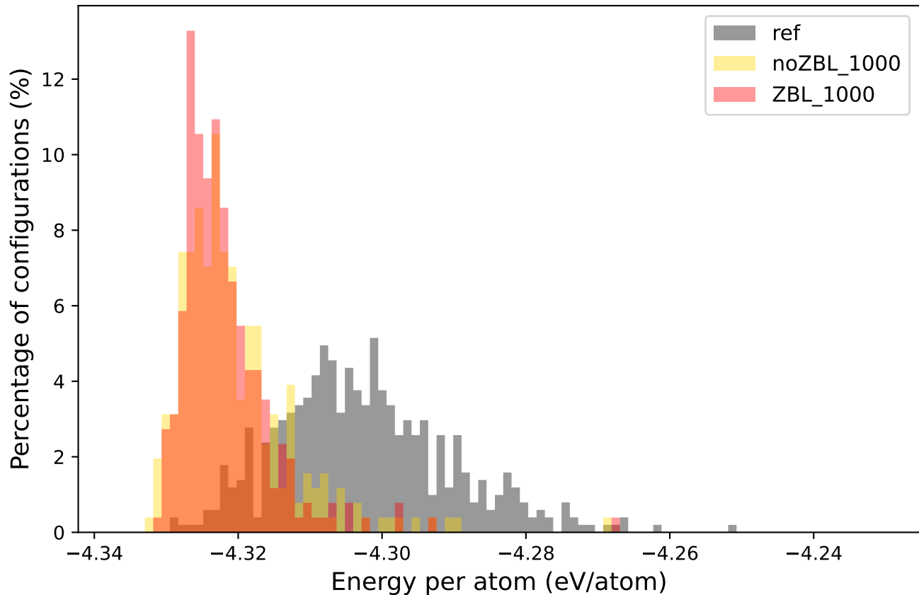
Energy distribution — Si111
