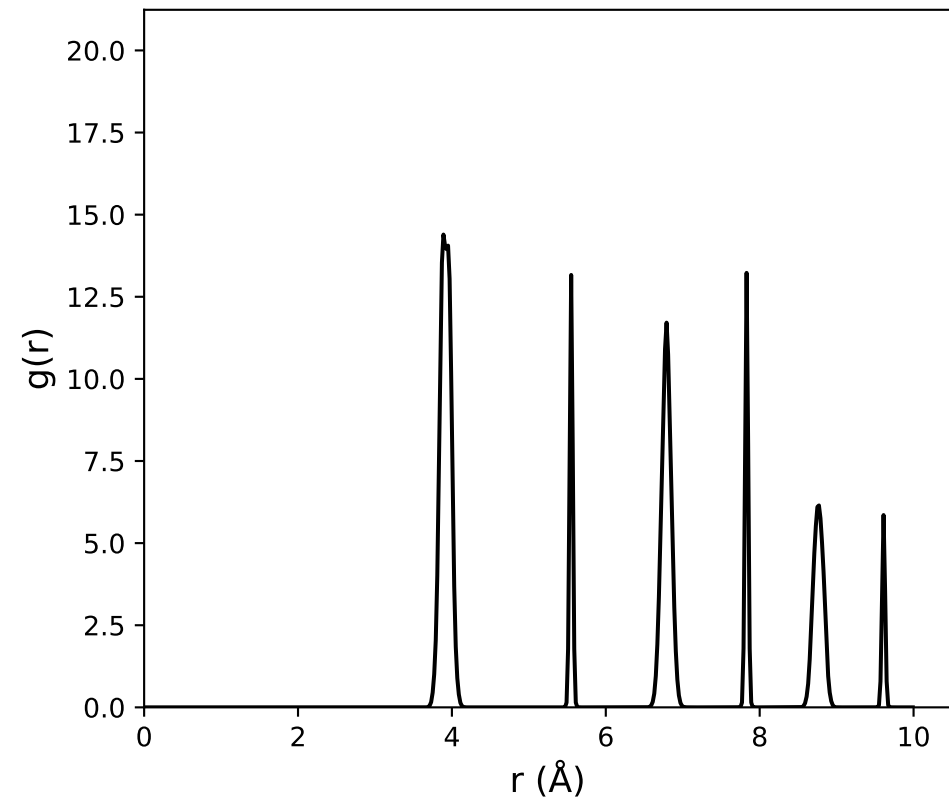
Ge-Ge
