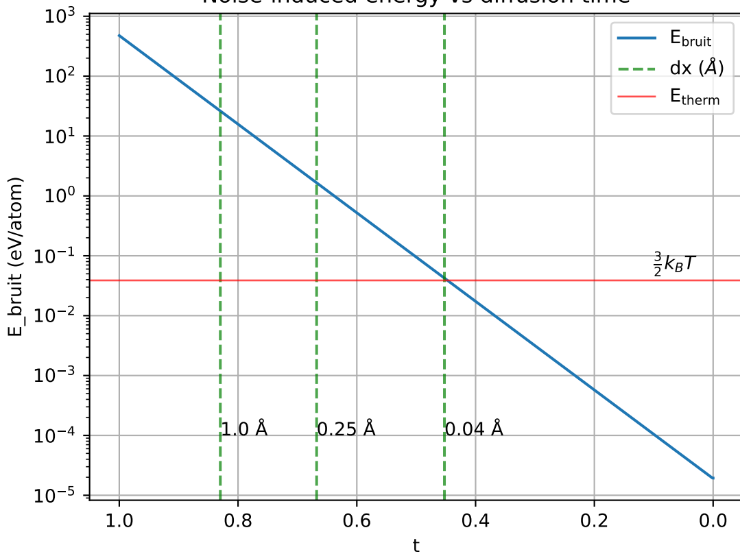
Noise-induced energy vs diffusion time
