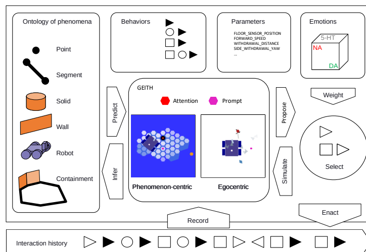
Figure 5.1. The Enactive Cognitive Architecture (ECA) from [GDMR24]
