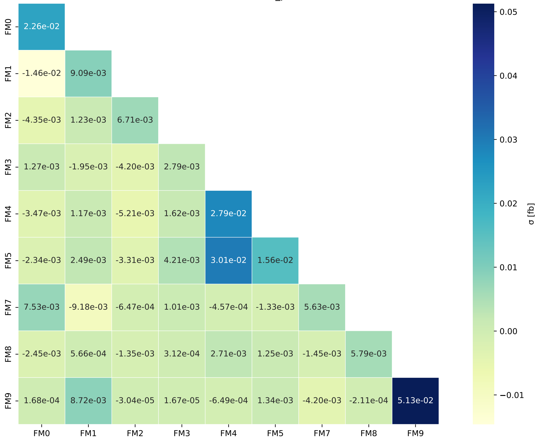
FM Cross Section Matrix (EFTDec_polarisation)
