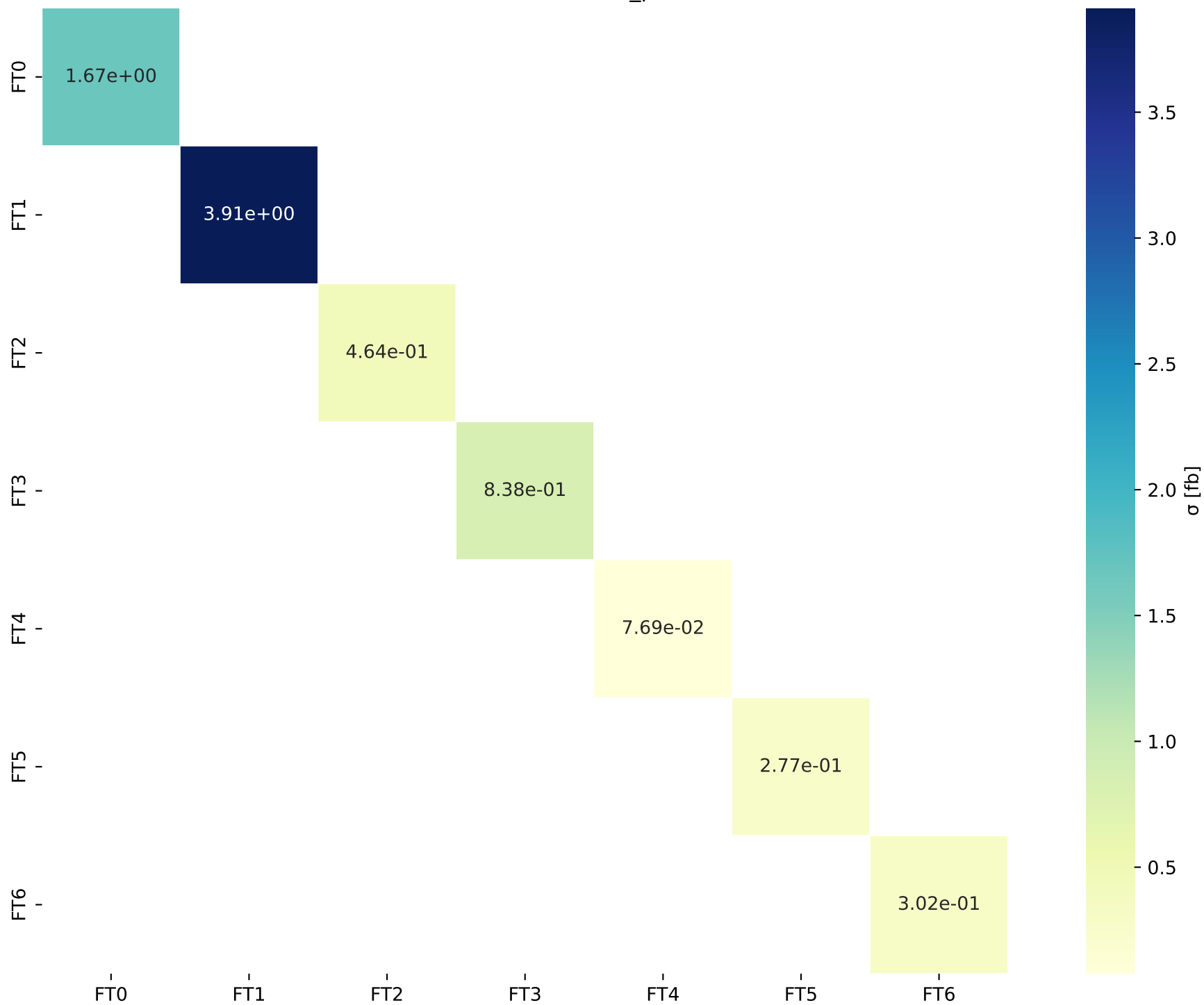
FT Cross Section Matrix (EFTDec_polarisation)
