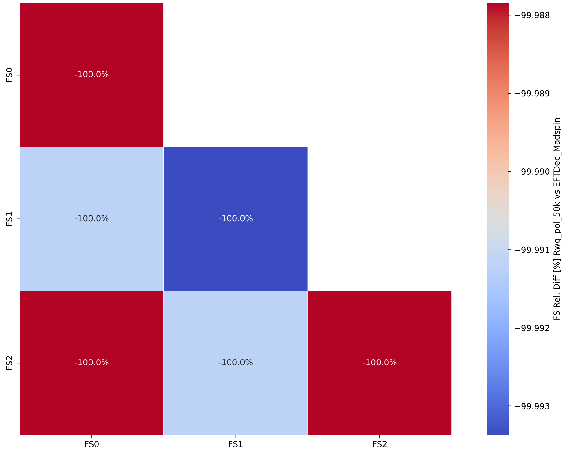
FS Rel. Diff [%] Rwg_pol_50k vs EFTDec_Madspin
