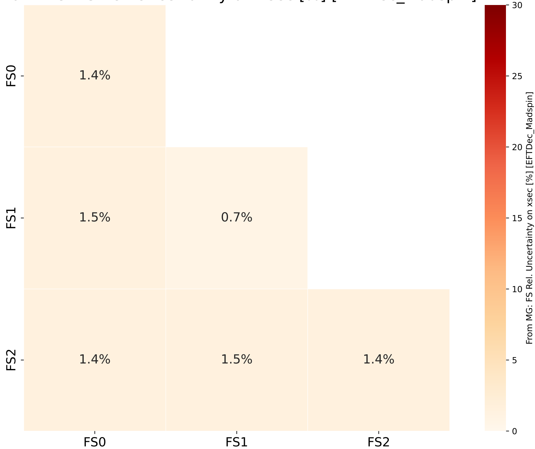
From MG: FS Rel. Uncertainty on xsec [%] [EFTDec_Madspin]
