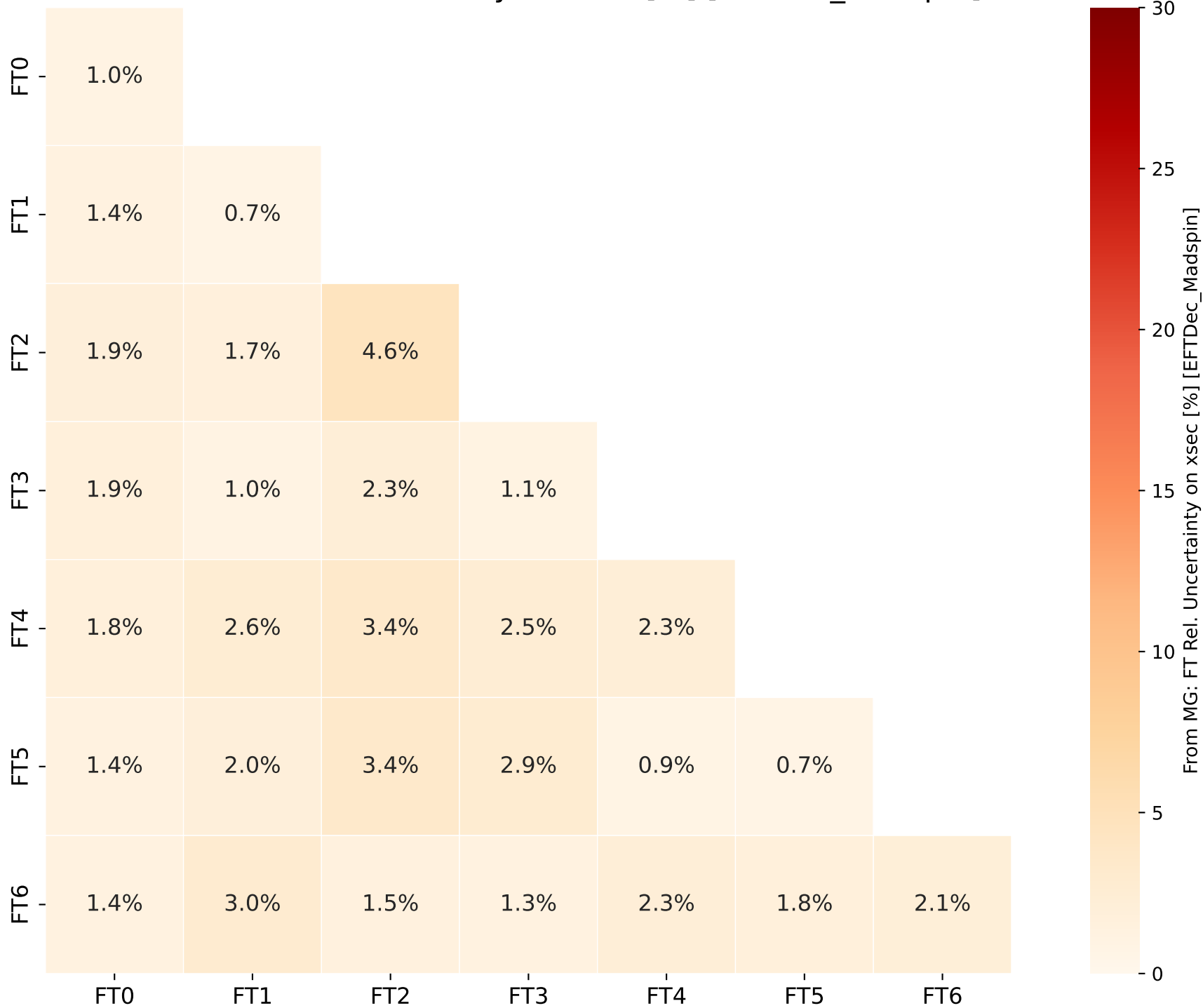
From MG: FT Rel. Uncertainty on xsec [%] [EFTDec_Madspin]
