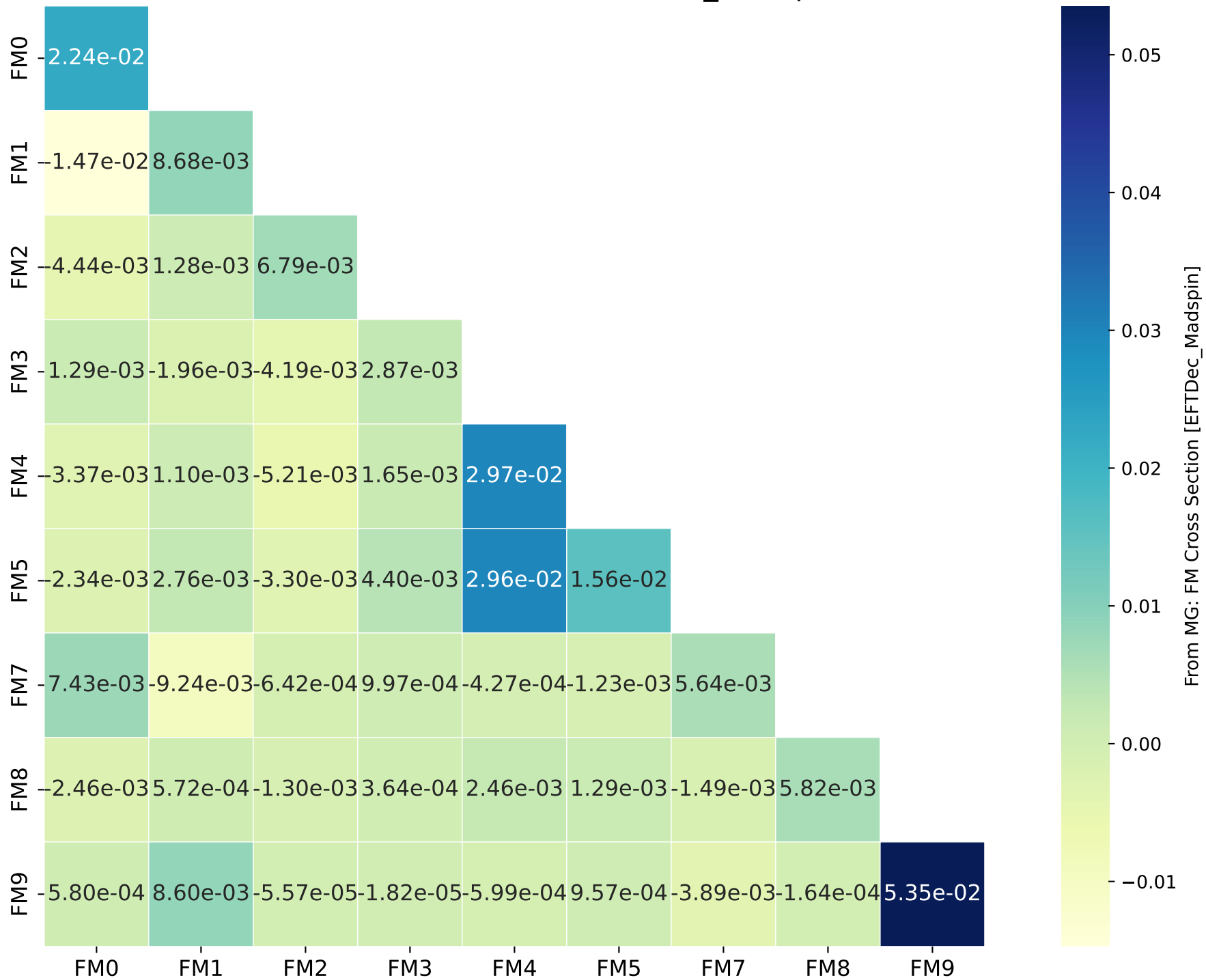
From MG: FM Cross Section [EFTDec_Madspin]
