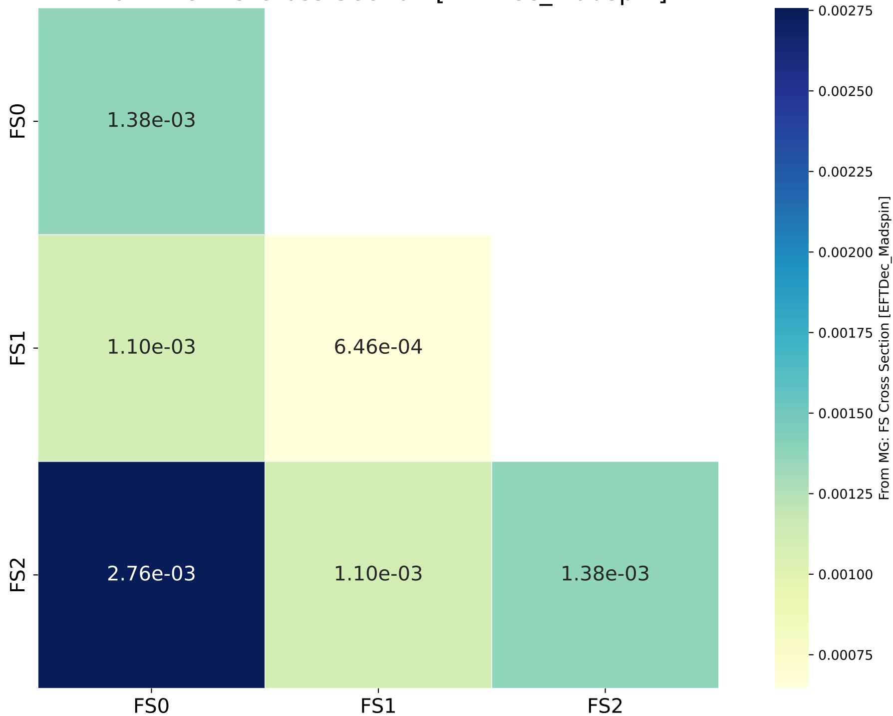
From MG: FS Cross Section [EFTDec_Madspin]
