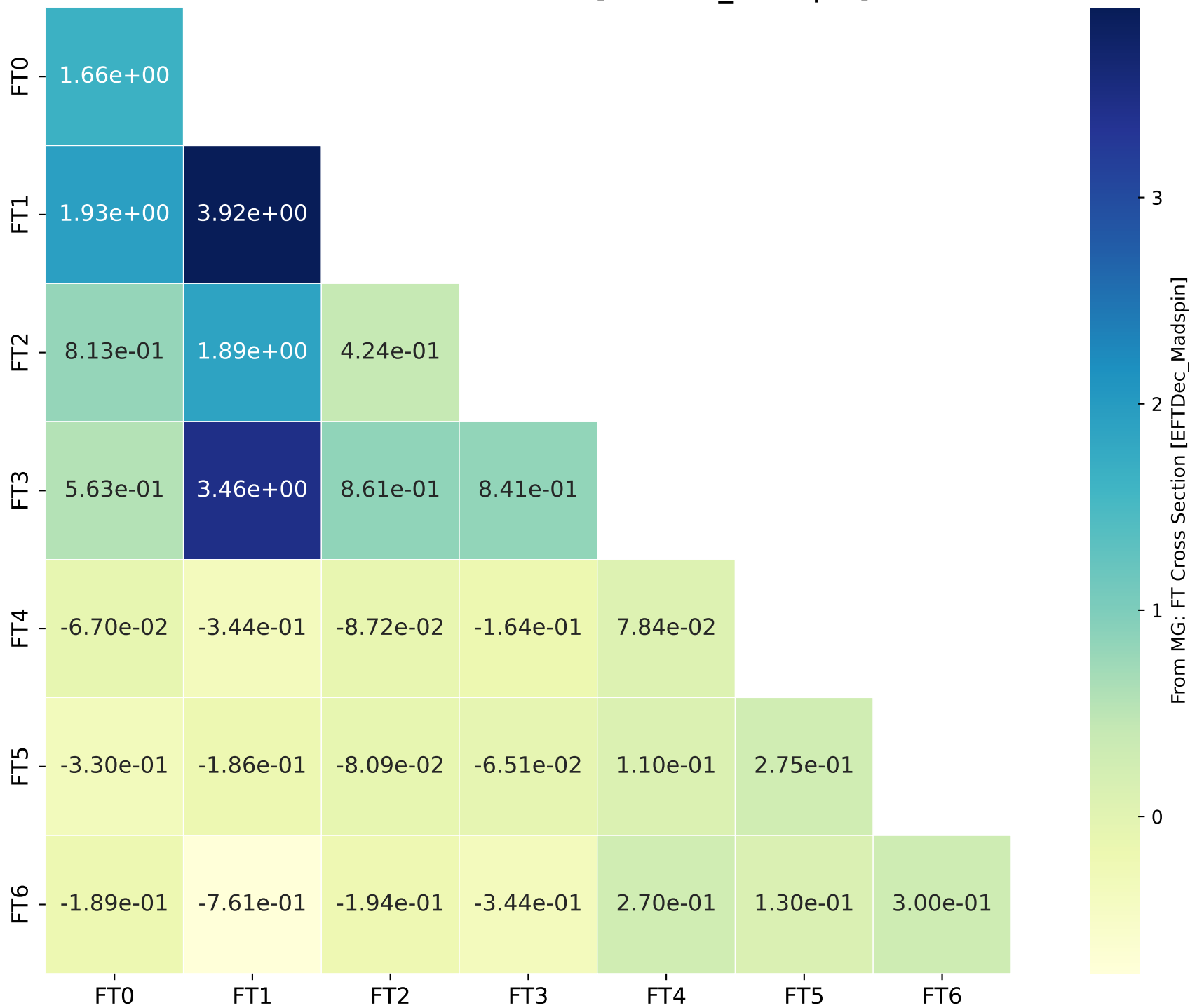
From MG: FT Cross Section [EFTDec_Madspin]
