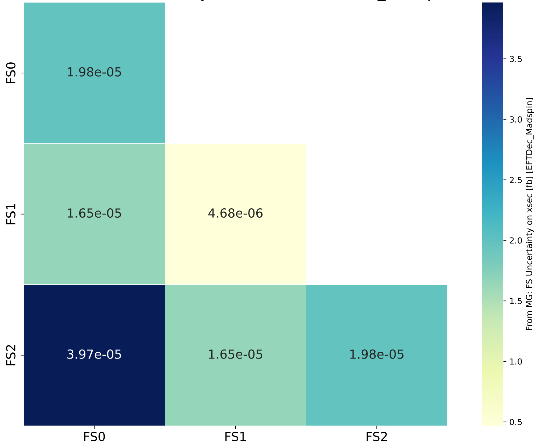
From MG: FS Uncertainty on xsec [fb] [EFTDec_Madspin]
