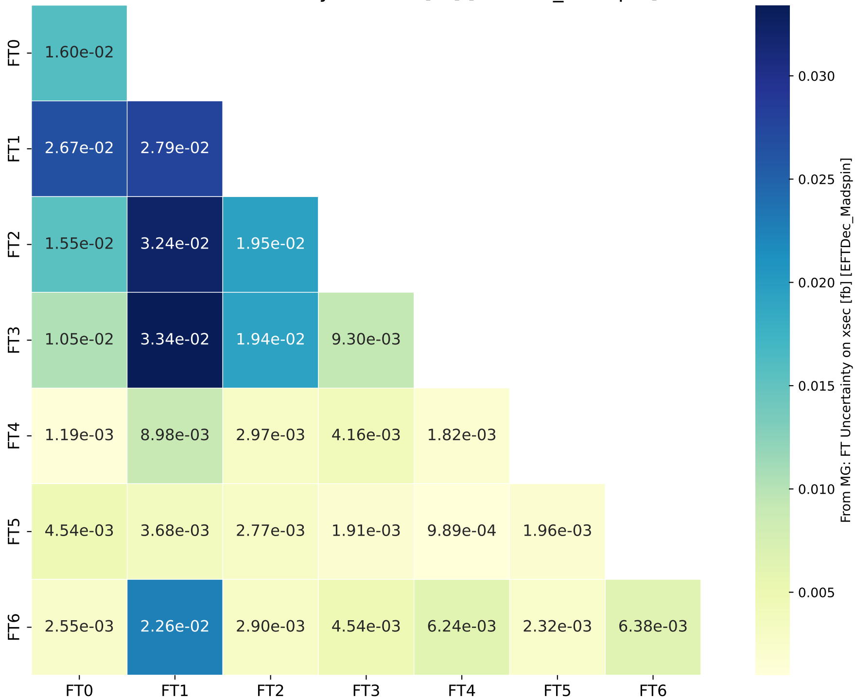
From MG: FT Uncertainty on xsec [fb] [EFTDec_Madspin]
