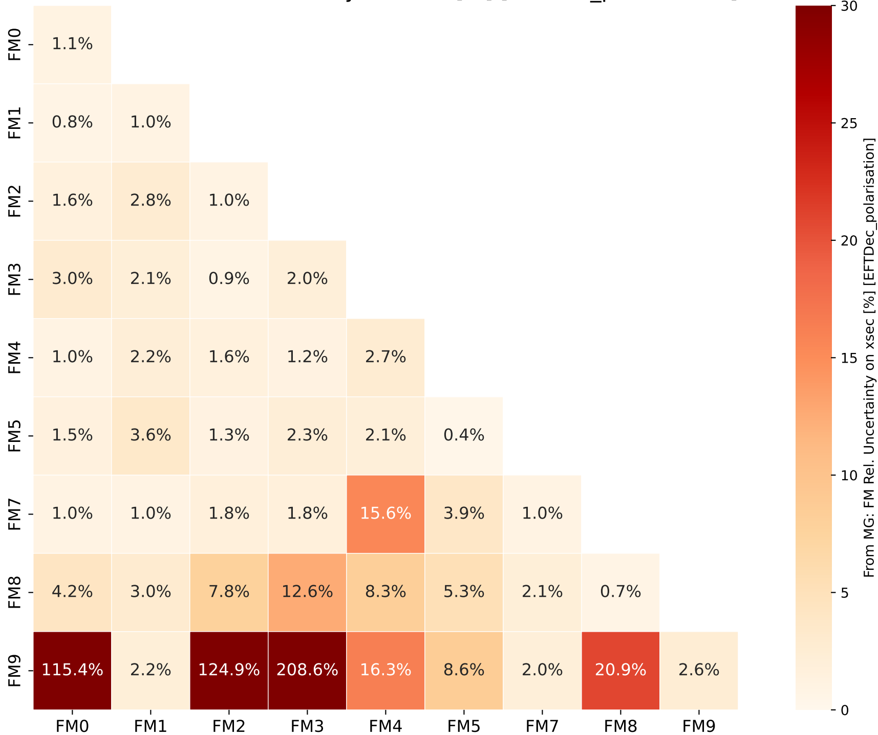
From MG: FM Rel. Uncertainty on xsec [%] [EFTDec_polarisation]
