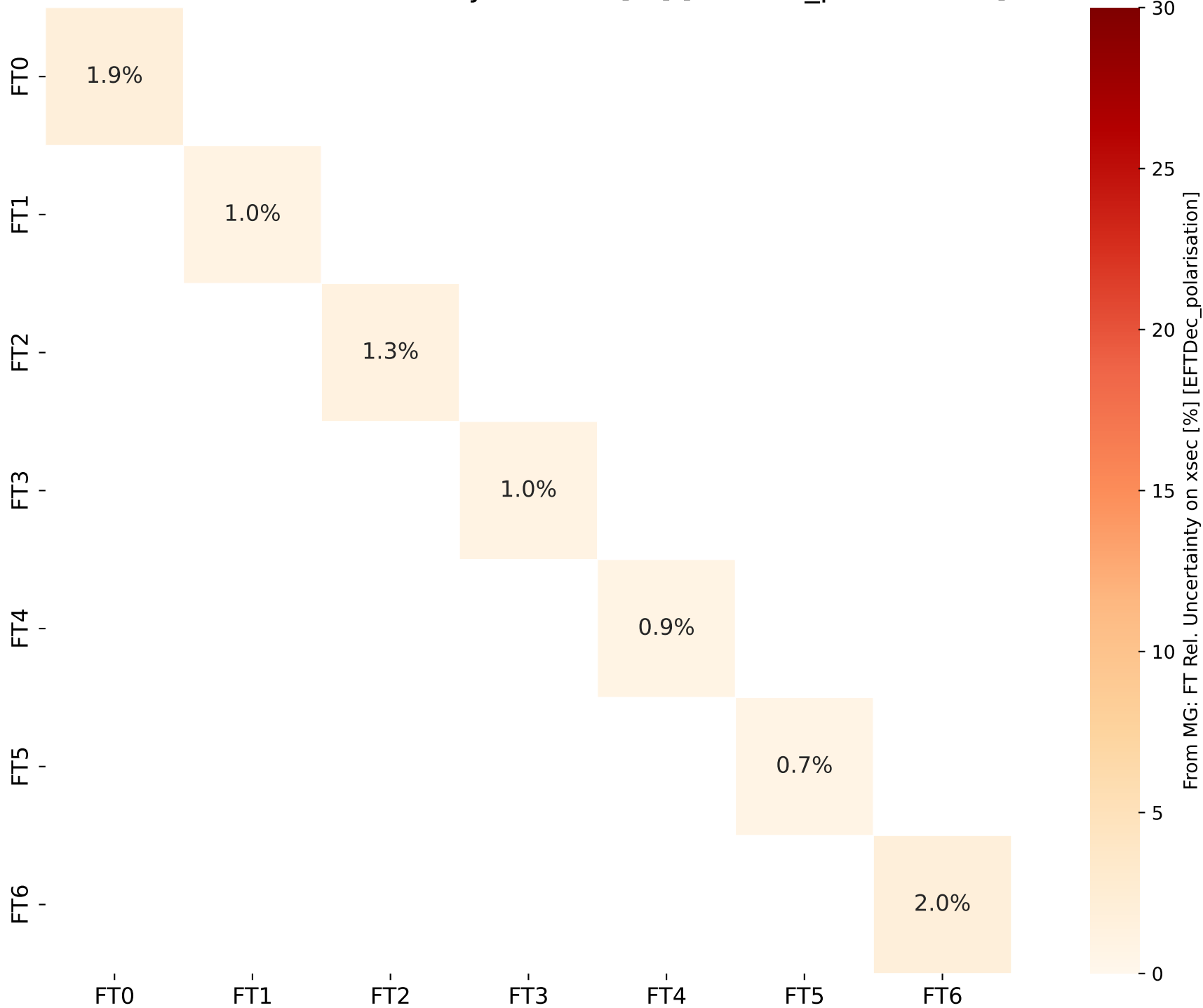
From MG: FT Rel. Uncertainty on xsec [%] [EFTDec_polarisation]
