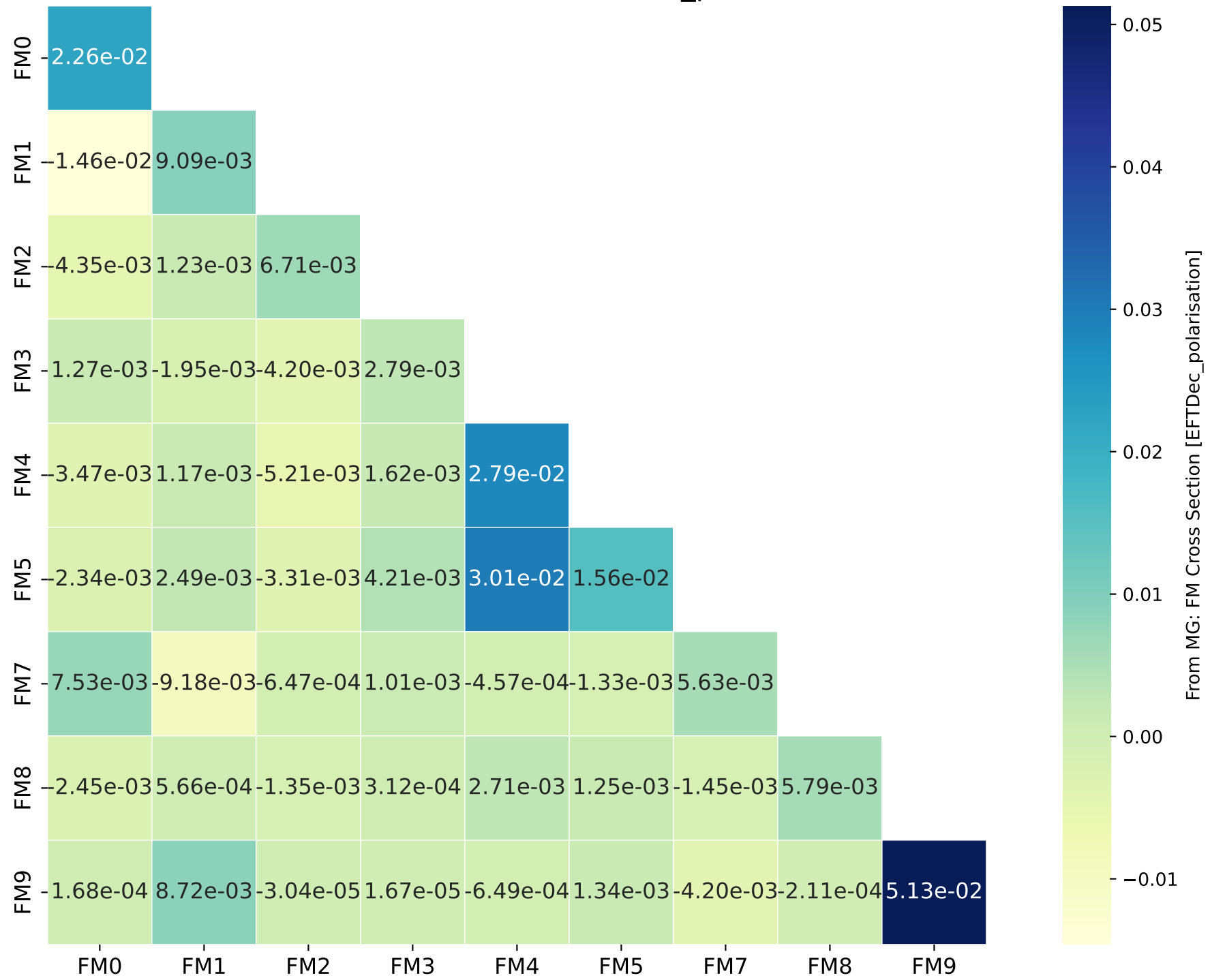
From MG: FM Cross Section [EFTDec_polarisation]
