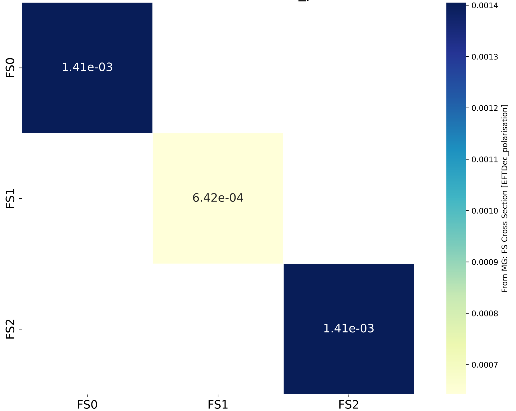
From MG: FS Cross Section [EFTDec_polarisation]
