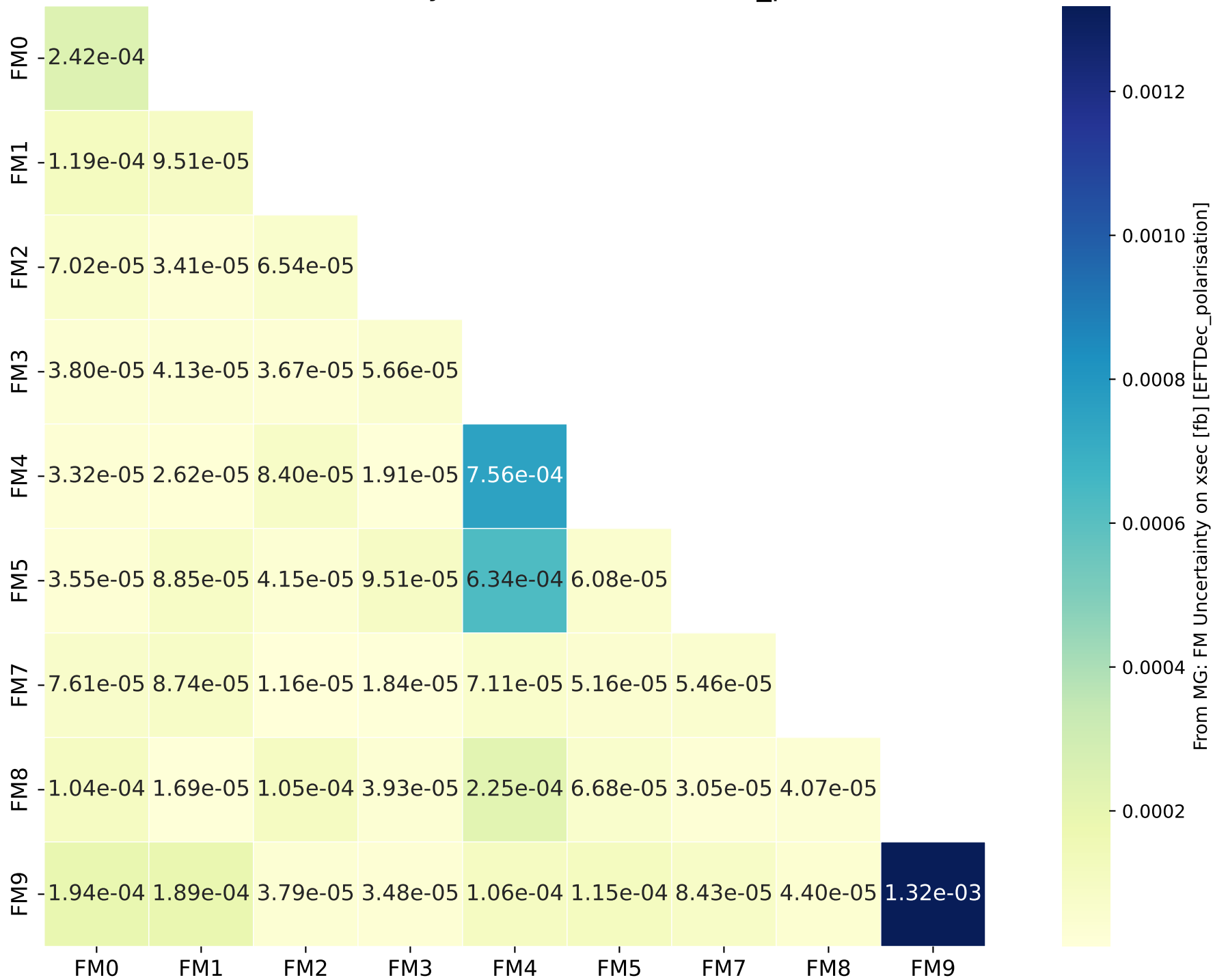
From MG: FM Uncertainty on xsec [fb] [EFTDec_polarisation]
